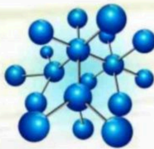
Tap Water H 2 O Cluster 20 to 25 Molecules
